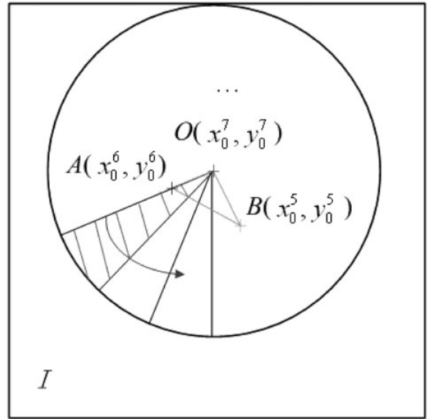
2 Image partitioning
